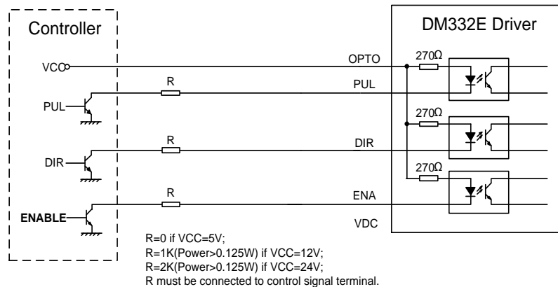
Figure 2: Connections to open-collector signal (common-anode)
