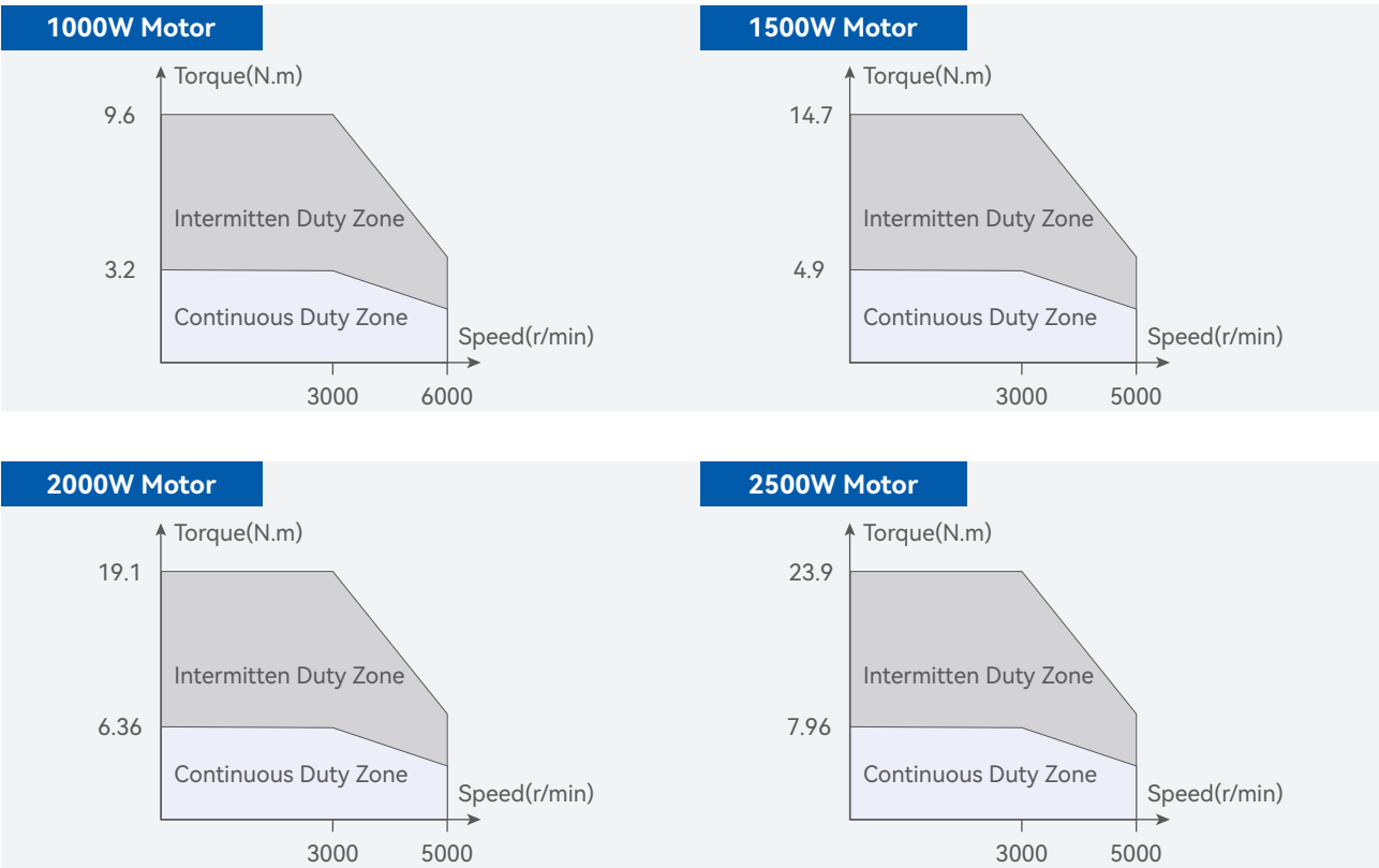
Speed-Torque characteristics
