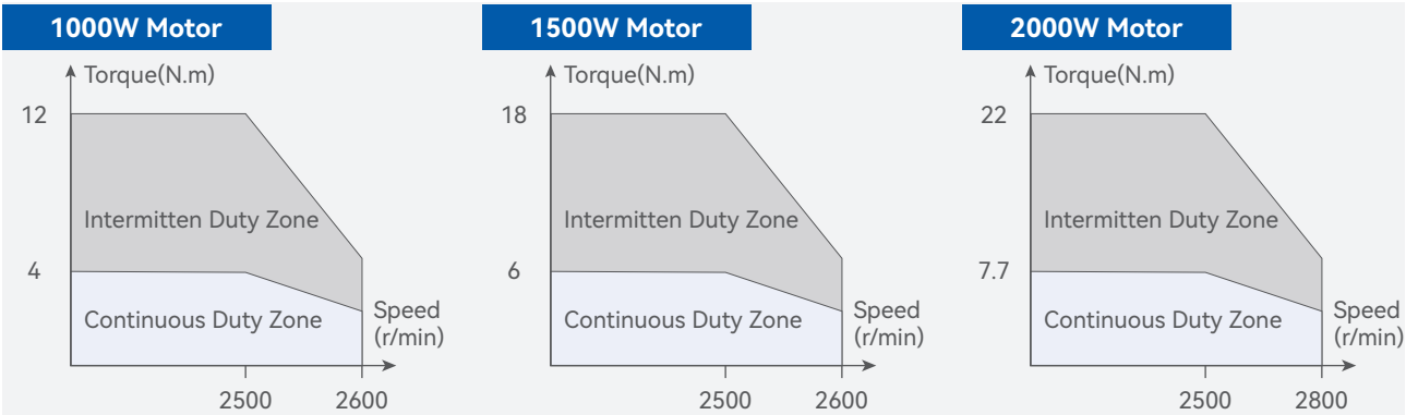
Speed-Torque characteristics
