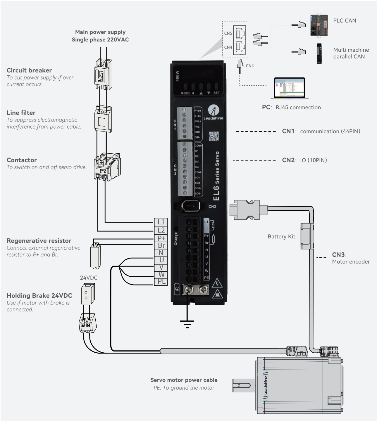
EL6-CAN & Peripheral Wiring Diagram
